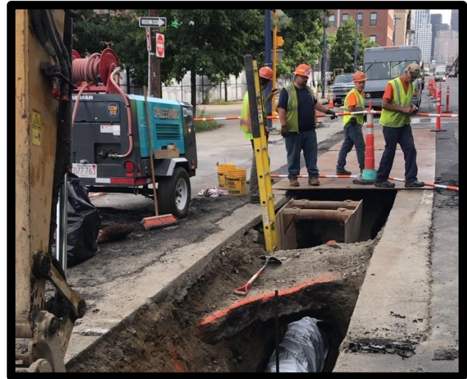
Water Main Installation Albany Street
