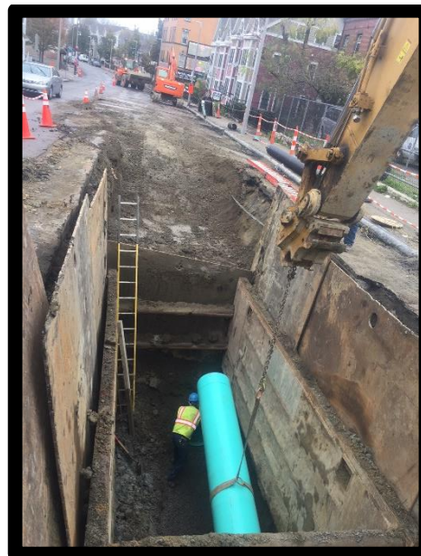
Dudley Street Installation of 24" Sewer Pipe
