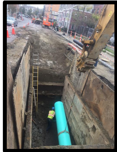
Dudley Street Installation of 24" Sewer Pipe
