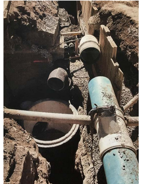
Phase II Temporary Drain Installation
