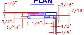
SECTION A-A COVER
