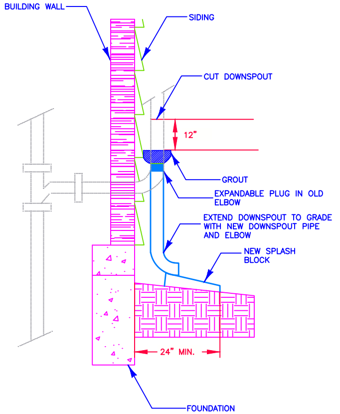
ELEVATION SIDE VIEW
