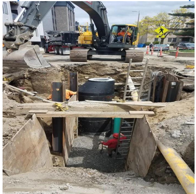
Typical Sewer Separation Project
