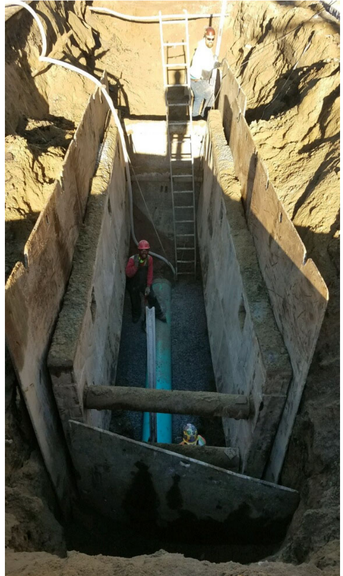
18-inch sewer installation on West Seventh Street
