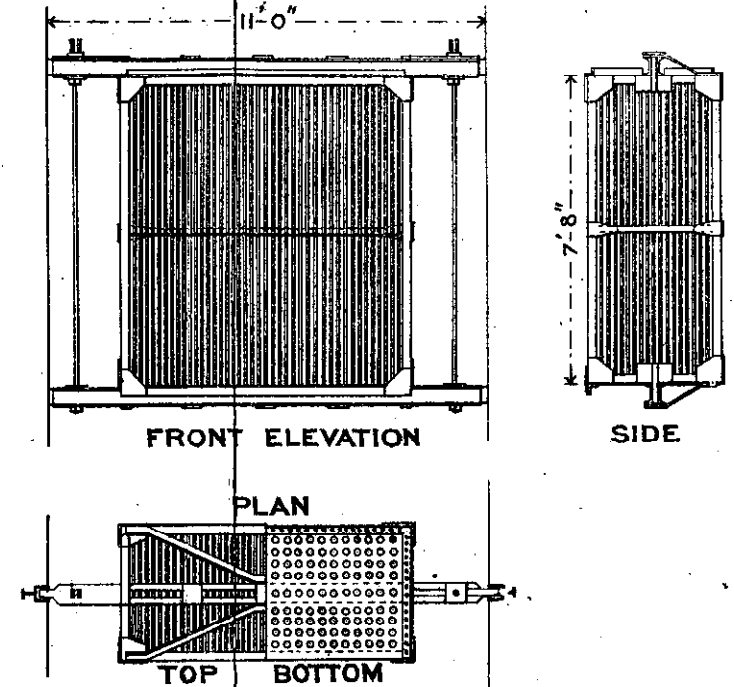
FILTH CAGES
