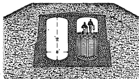
TRANSVERSE SECTION OF DEPOSIT SEWERS AND END VIEW OF SCRAPER. FIG. 7
