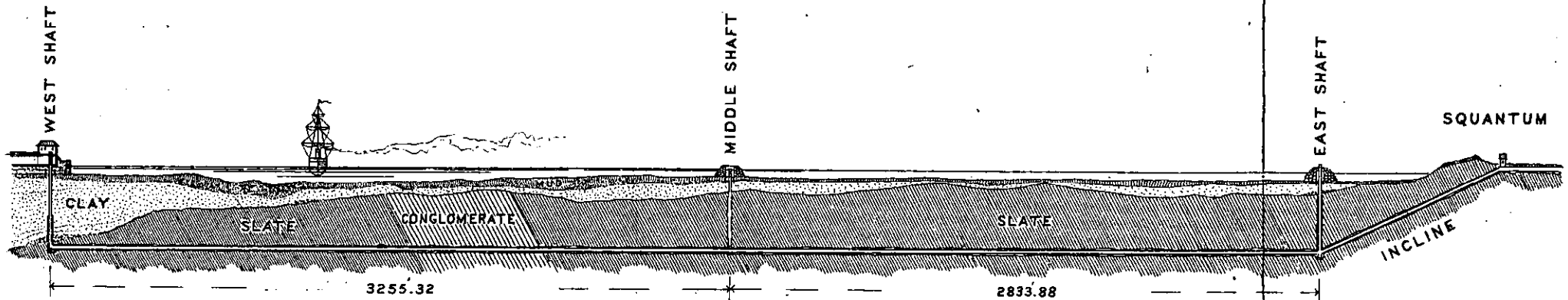
LONGITUDINAL SECTION OF TUNNEL
