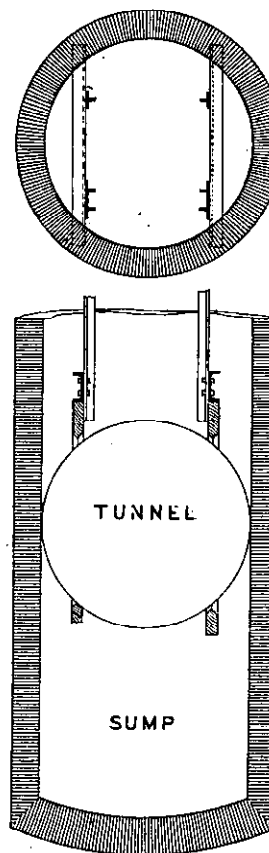
DETAIL SECTIONS OF EAST SHAFT SHOWING BEAMS AND GUIDES
