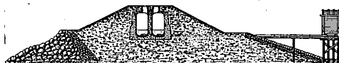
OLD HARBOR PIER CROSS SECTION. FIG. 5
