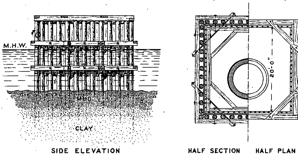
BULKHEADS ABOUT SHAFTS
