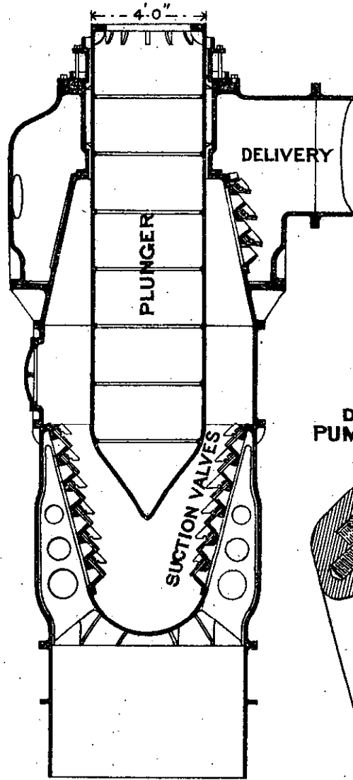
LEAVITT PUMP
