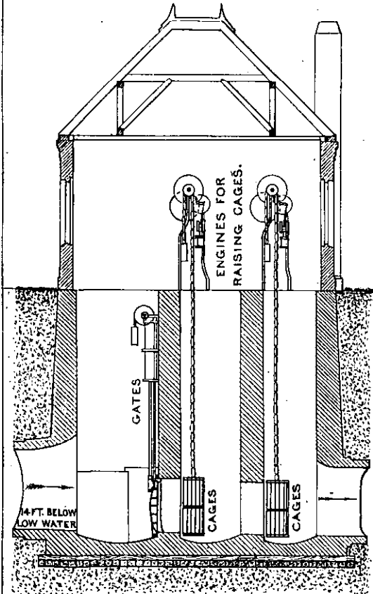
SECTION THROUGH FILTH HOIST AND CAGES.
