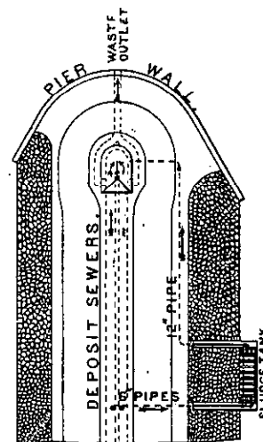
OLD HARBOR PIER PLAN AT END. FIG. 3
