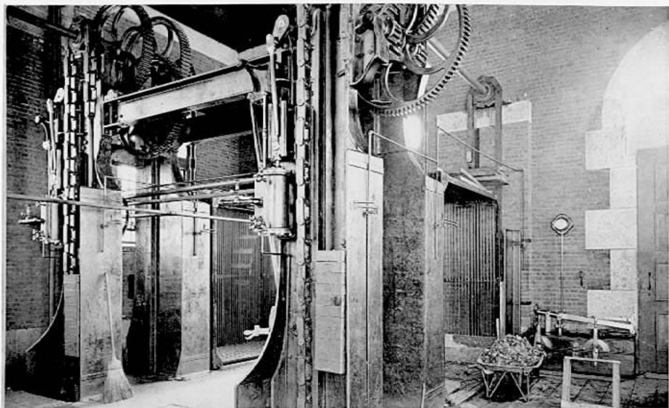
Interior of Filth-Hoist with one pair of cages raised.
