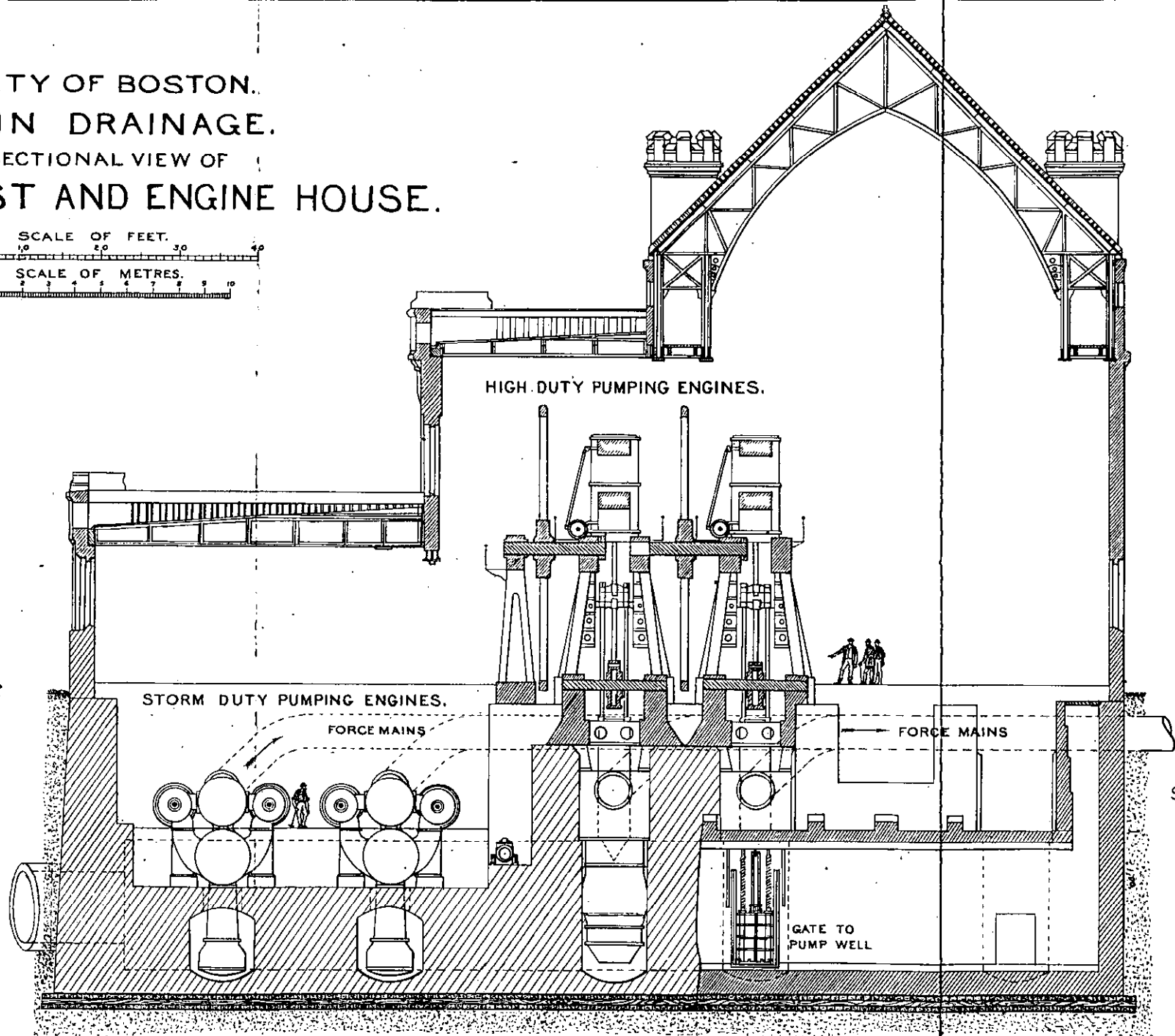
SECTION THROUGH PUMP WELLS.
