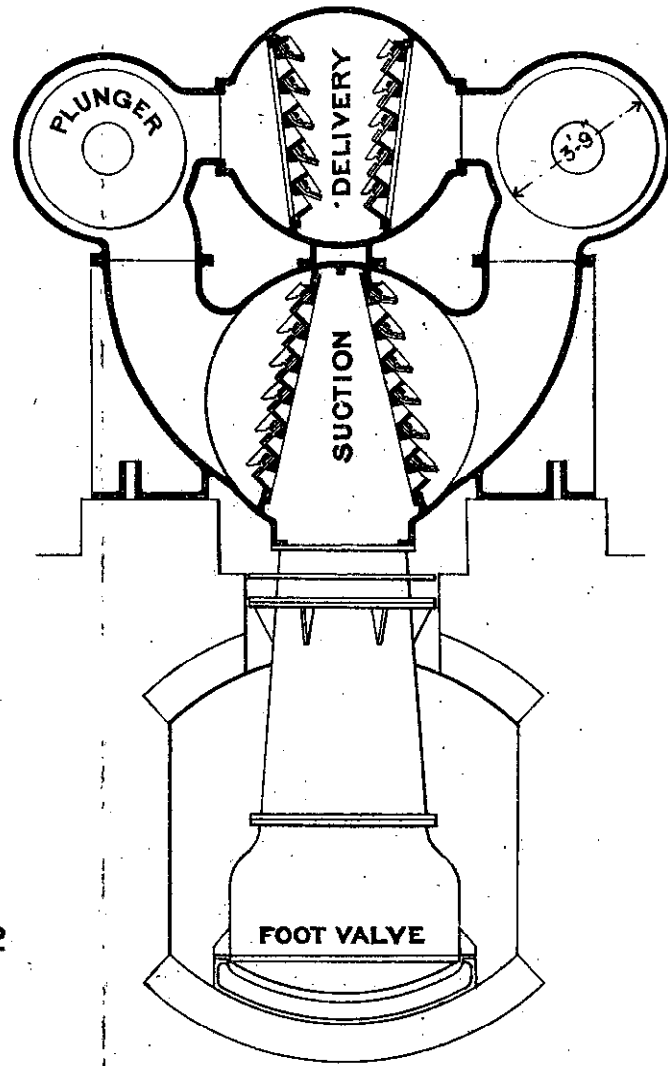
WORTHINGTON PUMP
