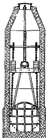
PENSTOCK GATE
