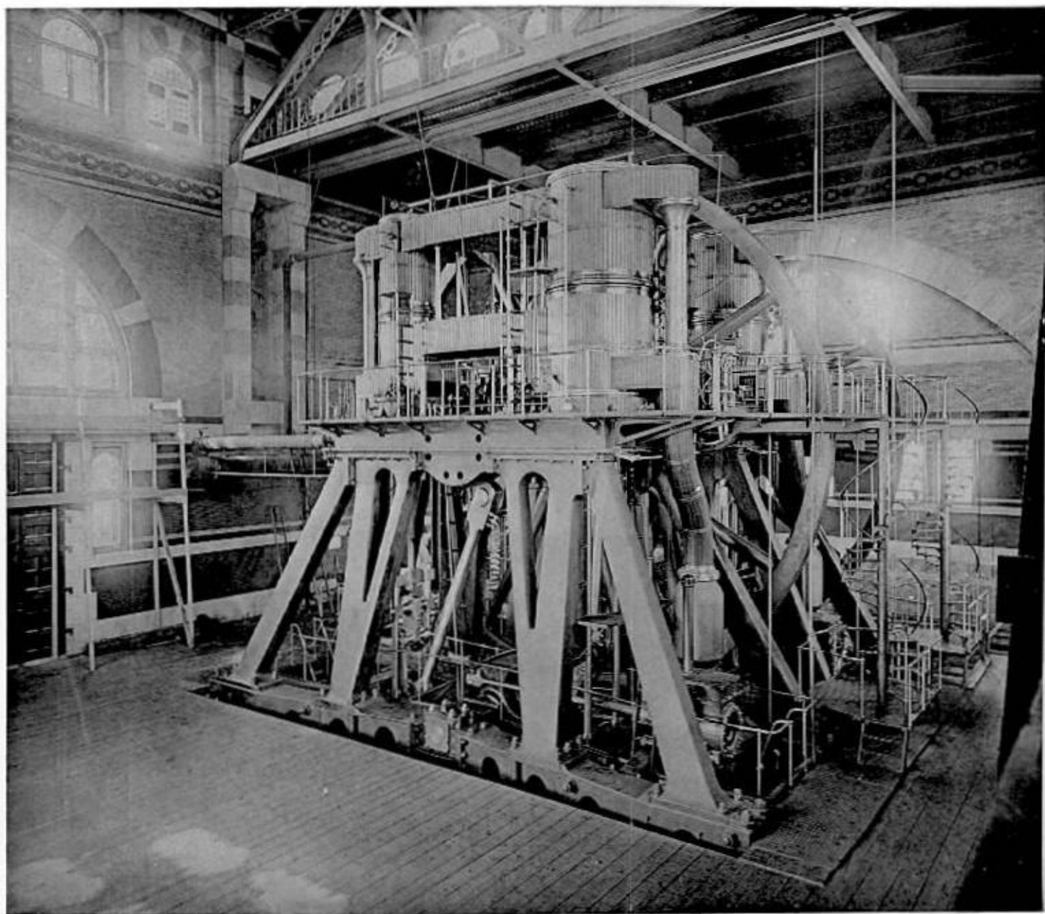
LEAVITT PUMPING ENGINES.
