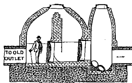
CONNECTION WITH VALE ST. SEWER.
