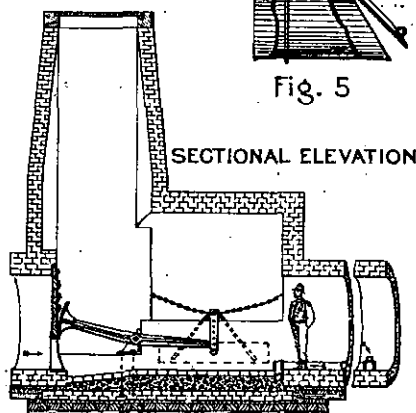
LARGE REGULATOR Fig. 9
