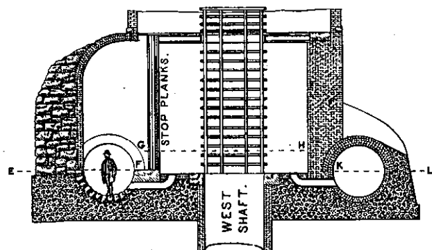
SECTIONAL ELEVATION ON LINES A.B.C.D. FIG. 2
