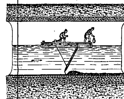
LONG SECTION OF DEPOSIT SEWER SHOWING SCRAPER. FIG. 8
