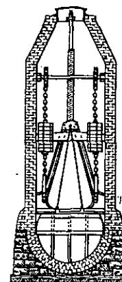
FLUSHING GATE
