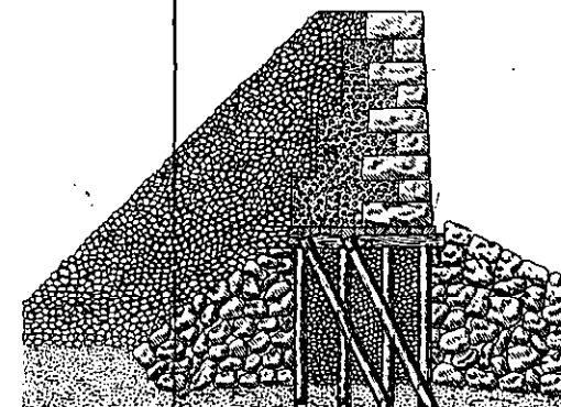
END WALL OF PIER. FIG. 4
