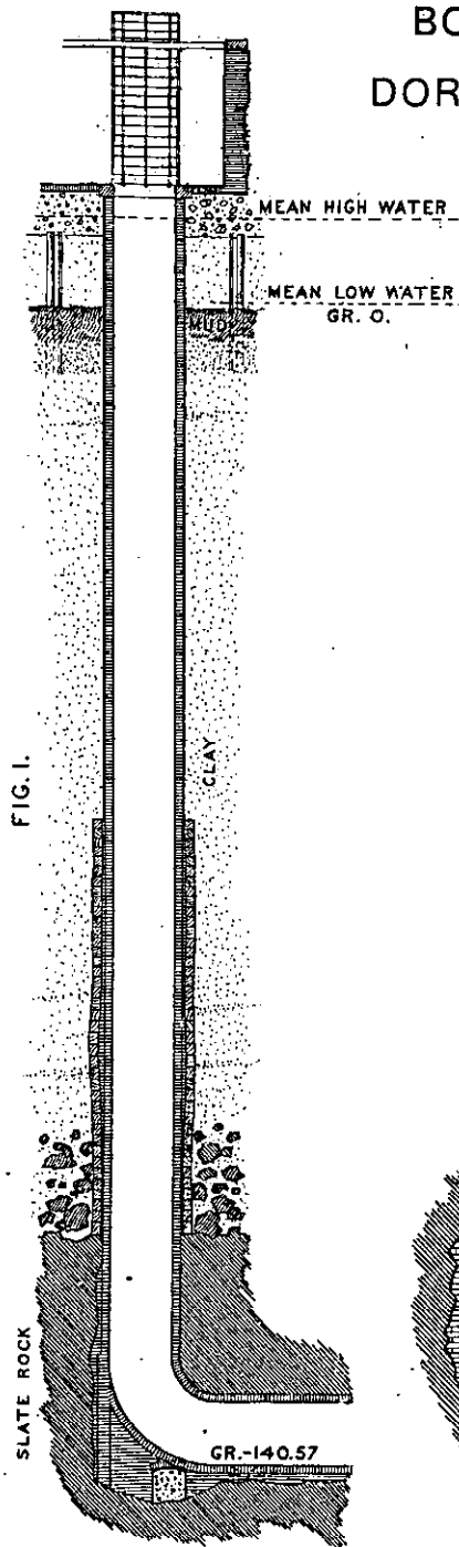
SECTION OF WEST SHAFT
