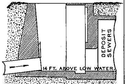
SECTION THROUGH PIPE CHAMBER.
