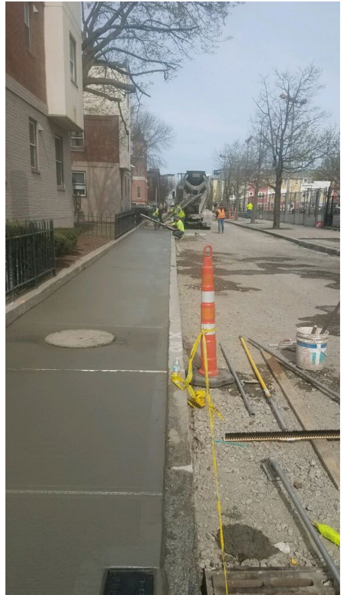
Concrete sidewalk replacement Flaherty Way
