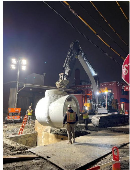
Drain tee manhole installation in Eagle Square
