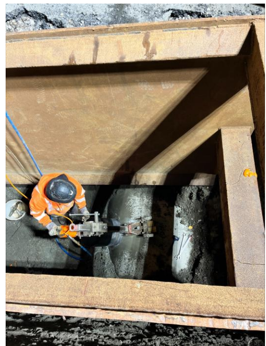
Coring 72" storm drain for catch basin connection in Eagle Square
